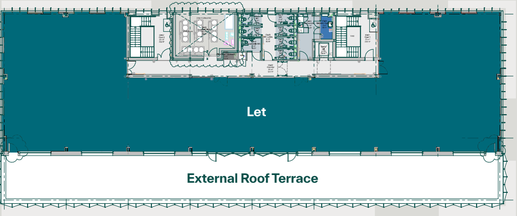
Third Floor
